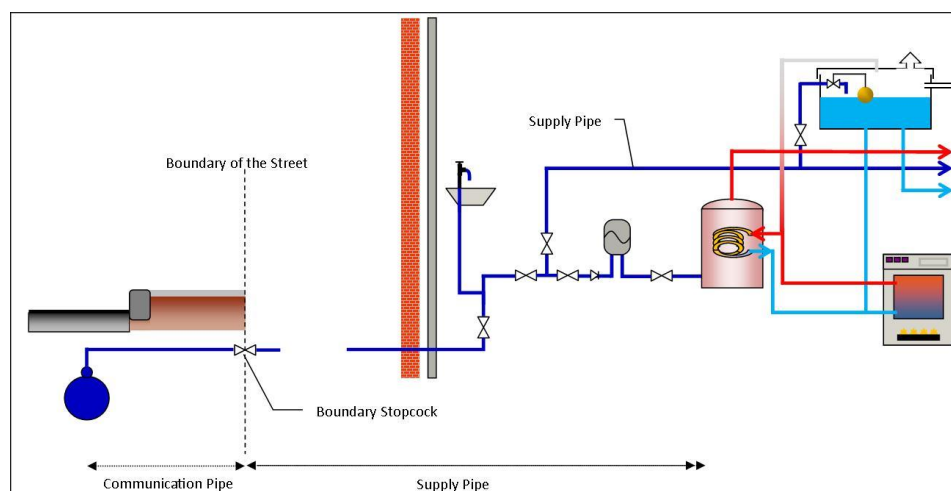
Diagram of Communication pipe and Supply pipes
